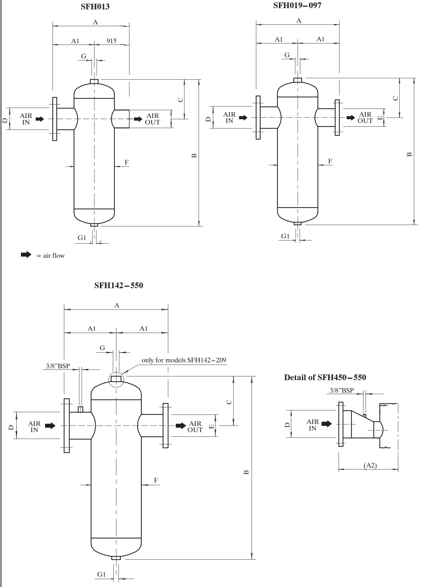
Fig. 1 A – Overall dimensions SFH
